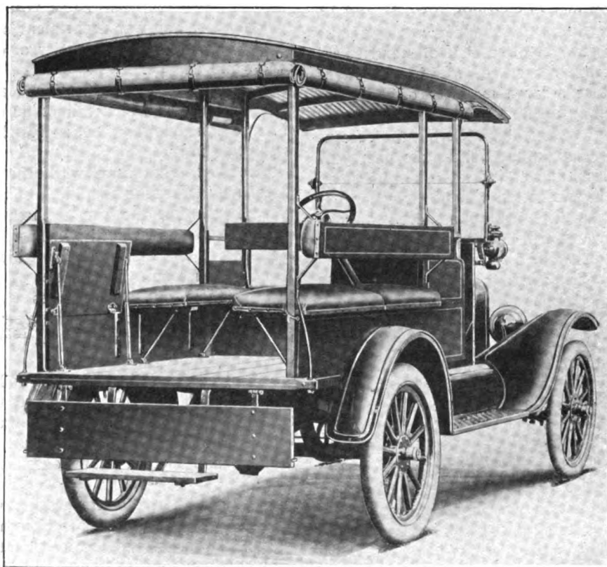
PASSENGER BODY Built by the Columbia Wagon Co., Columbia, Pa.
